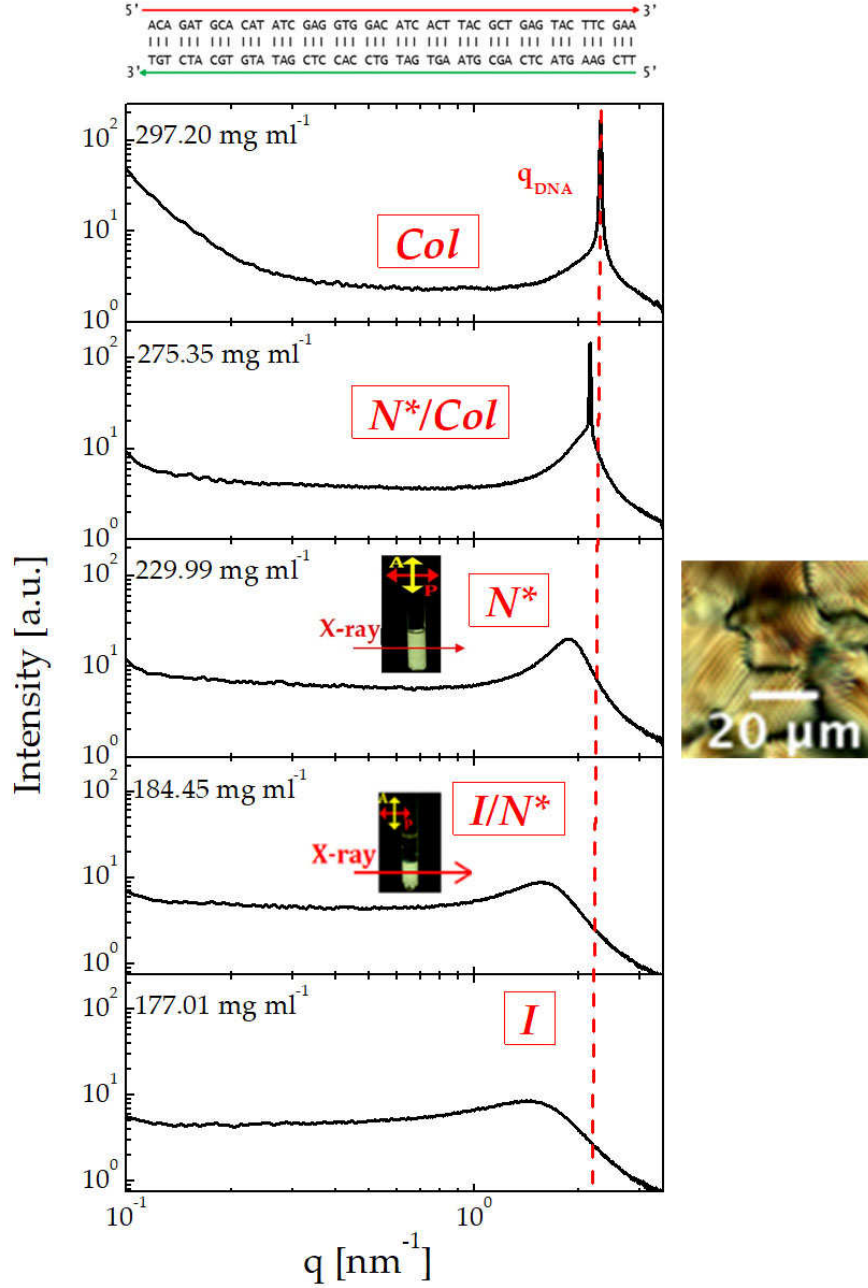
FIGURE 5.3: X-ray scattering patterns of 48 bp long F-DNA at concentrations (from top to the bottom) c = 297.2, 275.35, 229.99, 184.45, and 177.01 \text{ mg ml}^{-1} . POM micrograph with typical fingerprint texture of N^* phase is shown on the right-hand side.
