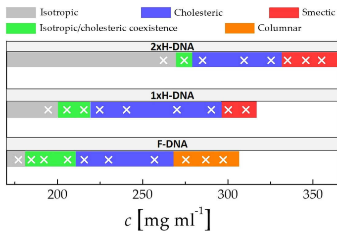
FIGURE 5.9: Phase diagram comparing dsDNA with no hairpins, 1xH-DNA and 2x-DNA.
