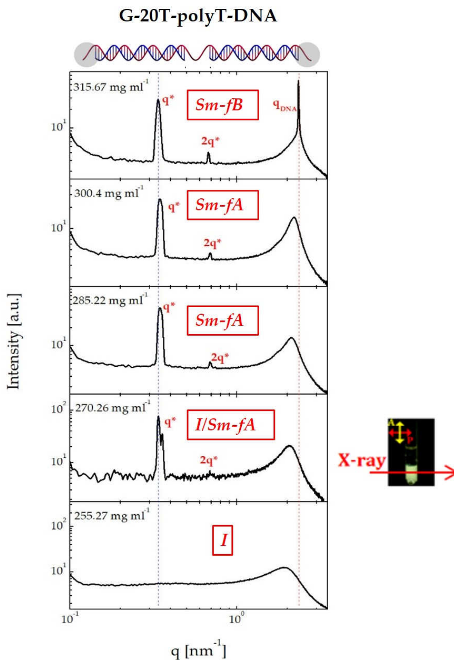
FIGURE 4.24: a) X-ray scattering profiles of G-20T-polyT-DNA at total DNA concentrations (from top to the bottom) c = 315.67, 300.4, 285.22, 270.26 , and 255.27 mg ml -1 . On the right-hand side is sample observed under crossed polarizers. The red arrow indicates part of the sample probed by the x-ray beam.
