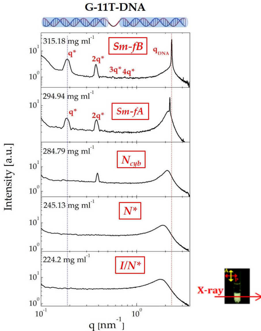
FIGURE 4.19: X-ray scattering profiles of G-11T-DNA duplexes at concentrations (from top to the bottom) c = 315.18, 294.94, 284.79, 245.13, and 224.2 \text{ mg ml}^{-1} . On the right-hand side is sample observed under crossed polarizers. The red arrow indicates part of the sample probed by the x-ray beam.
