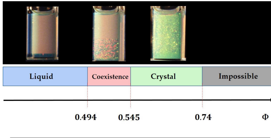
FIGURE 2.9: Phase transitions in hard spheres as a function volume fraction.
