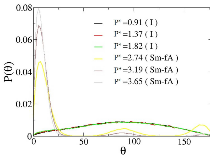
FIGURE 4.13: Distribution of angles between two cylinders of the same G-DNA duplex at different pressures for isotropic ( \beta P v_0 = 0.91 , 1.37, and 1.82) and smectic phase ( \beta P v_0 = 3.19 and 3.65).
