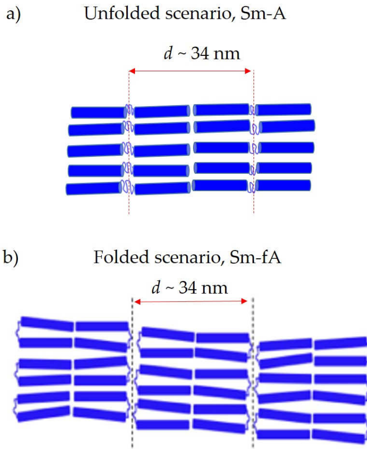
FIGURE 4.7: Schematic representation of two possible molecular arrangements within the smectic-A phase. a) Unfolded scenario in which G-DNA duplexes are in an unfolded layer-like arrangement. b) Folded scenario in which G-DNA duplexes are folded and stacked on top of one another.
