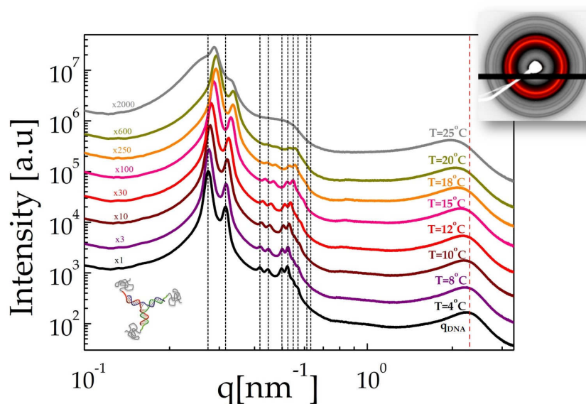
FIGURE 6.22: X-ray scattering profiles of Y-DNA with PNIPAm 19 kDa attached on all three arms at concentration c=213 \text{ mg ml}^{-1} , at T=4, 8, 10, 12, 15, 18, 20 , and 25^\circ\text{C} . The expected peak positions for the OBDG morphology are shown with dashed grey lines. Dashed red line shows the temperature dependence of the q_{\text{DNA}} peak. The 2D scattering pattern at 4^\circ\text{C} is shown on the top right-hand side.
