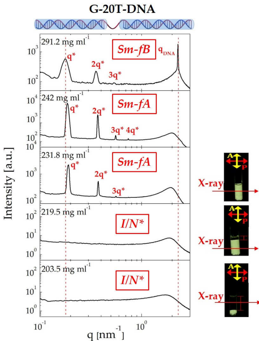
FIGURE 4.4: X-ray scattering profiles of G-20T-DNA duplexes at concentrations (from top to the bottom) c = 291.2, 242, 231.8, 219.5, and 203.5 \text{ mg ml}^{-1} . On the right-hand side are samples observed under crossed polarizers. The red arrow indicates part of the sample probed by the x-ray beam.
